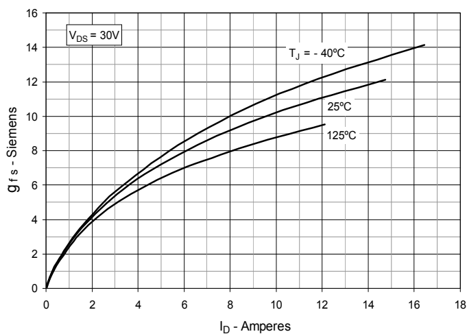
Fig. 10. Transconductance
