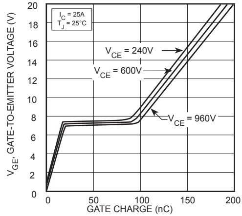
FIGURE 11, Gate charge vs. Gate-to-Emitter Voltage
