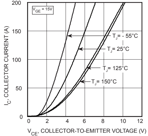
FIGURE 3, Output Characteristics
