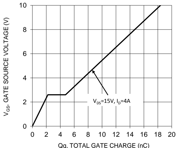
Figure 12 Gate Charge
