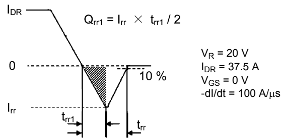
Fig. 6.4.1 t_{rr} Waveform
