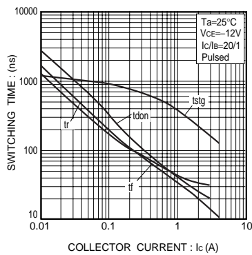
Fig.7 Switching time
